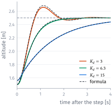
Step responses: simulator and formula
