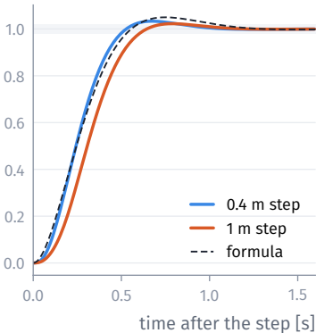
Response, as a fraction of the step
