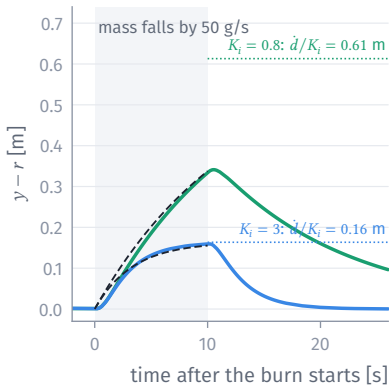
Height above the setpoint, load ramping
