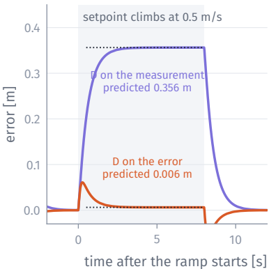
Error while the setpoint ramps (I off)
