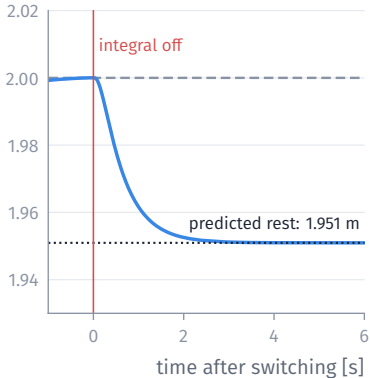
P and D remain: it rests 4.9 cm low
