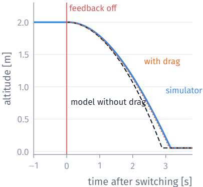
Open loop: the drone sinks
