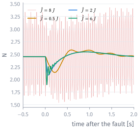
Thrust of motor 1 around the fault
