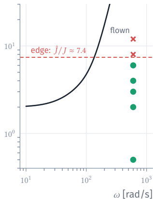
1 + 1/|FG|
