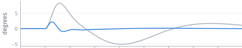
The three parts of the INDI command, roll axis
