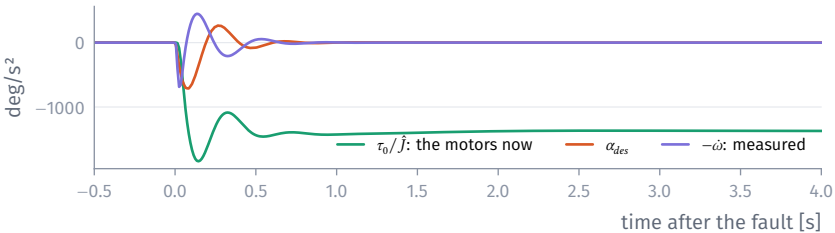
The three parts of the INDI command, roll axis
