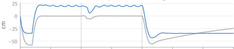
Error in altitude (the mass jumps from 1.0 to 1.5 kg at 20 s)
