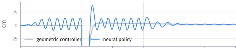
Error in altitude (the mass jumps from 1.0 to 1.5 kg at 20 s)
