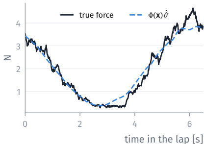
Disturbance force x , last lap
