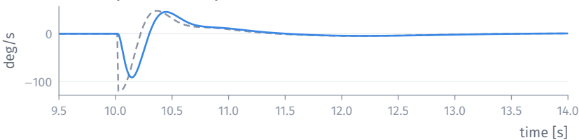
Rate loop (PID, 1 kHz): pitch rate
