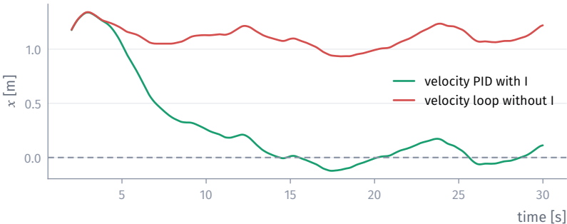
Position downwind in a 5 m/s wind (setpoint x = 0 )
