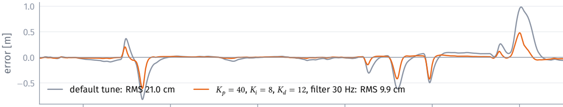
The gust challenge: altitude error, same wind for both runs (seed 4242)
