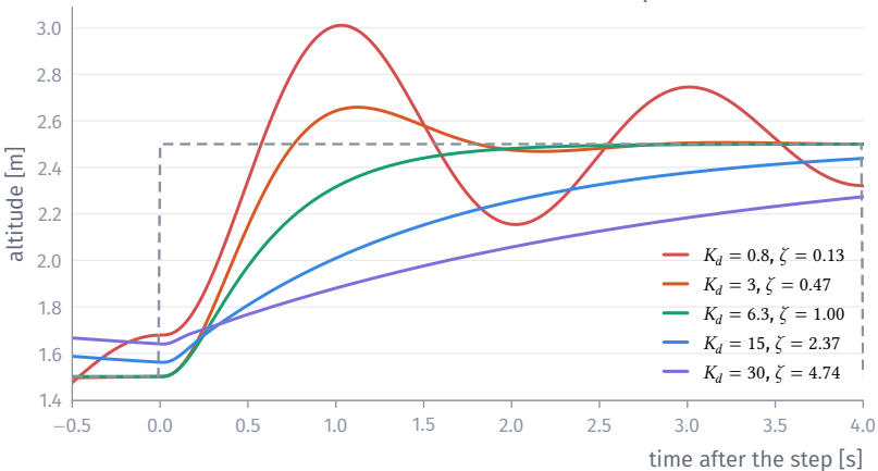
One upward step of the square wave, five dampers ( K_p = 10 )
