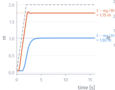
Altitude, P only, no feedforward
