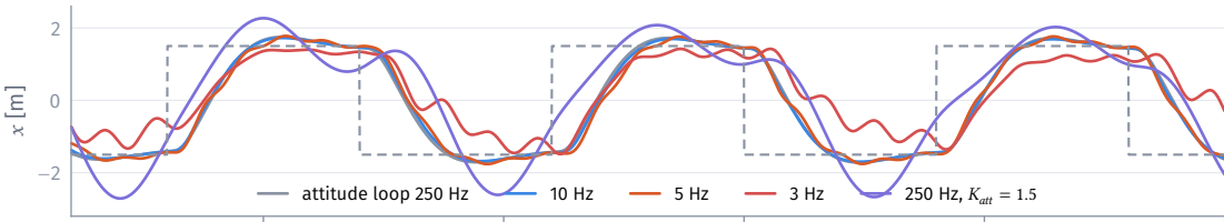
A square wave of \pm 1.5 m in x : position
