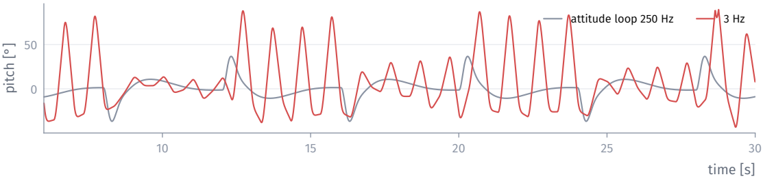
Pitch angle: the slow attitude loop swings up to 80^\circ
