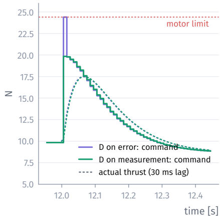
Zoom on the step at 12 s: total thrust
