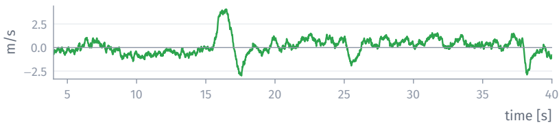
Vertical wind — what the controller never sees
