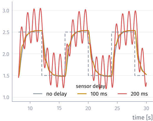
Sensor delay at 250 Hz
