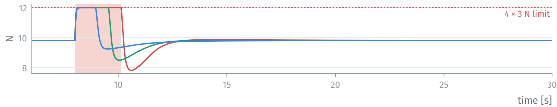
Total thrust (red shading: output saturated, no anti-windup)
