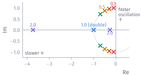
Poles s/\omega_n as \zeta grows
