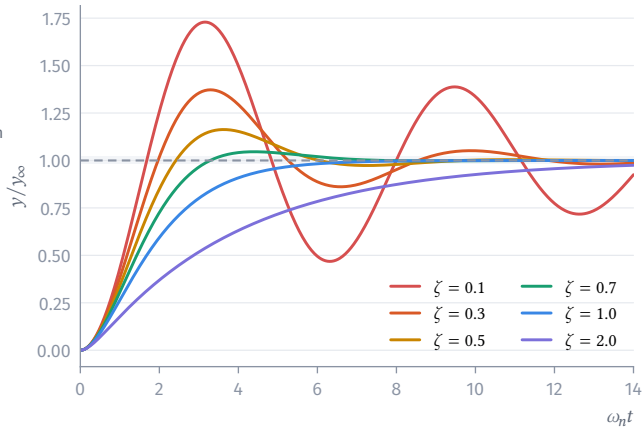
Step responses
