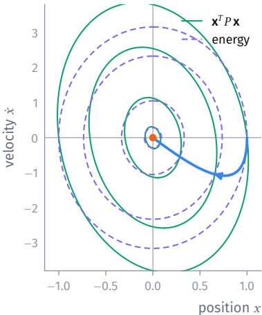
Two Lyapunov functions
