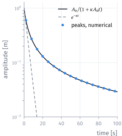
Drag alone: decay like 1/t
