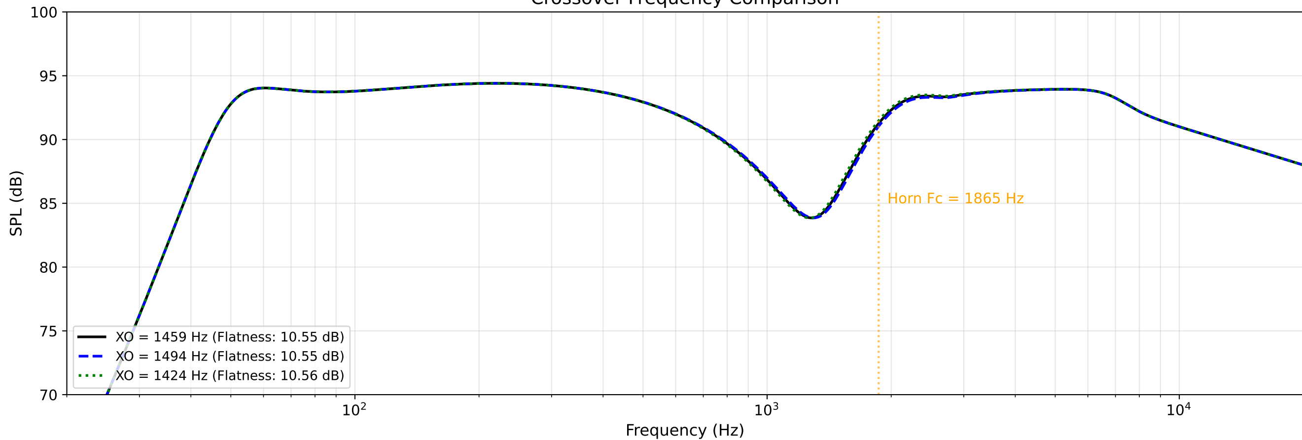
Crossover Frequency Comparison
