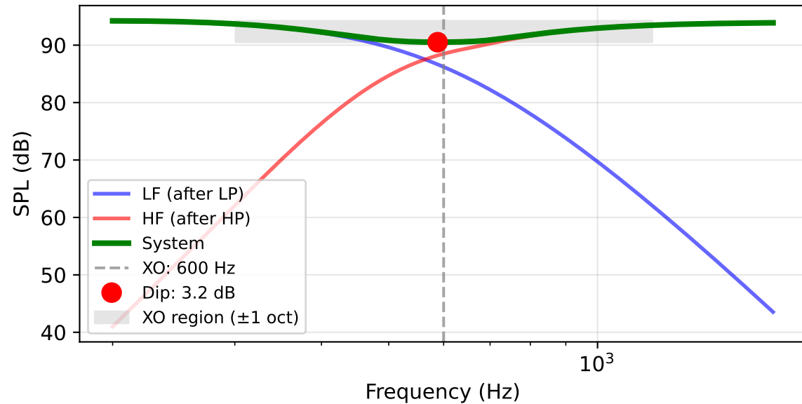
Crossover Region Detail (200-1800 Hz)
