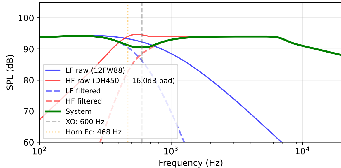
Optimized System: Individual Driver Responses
