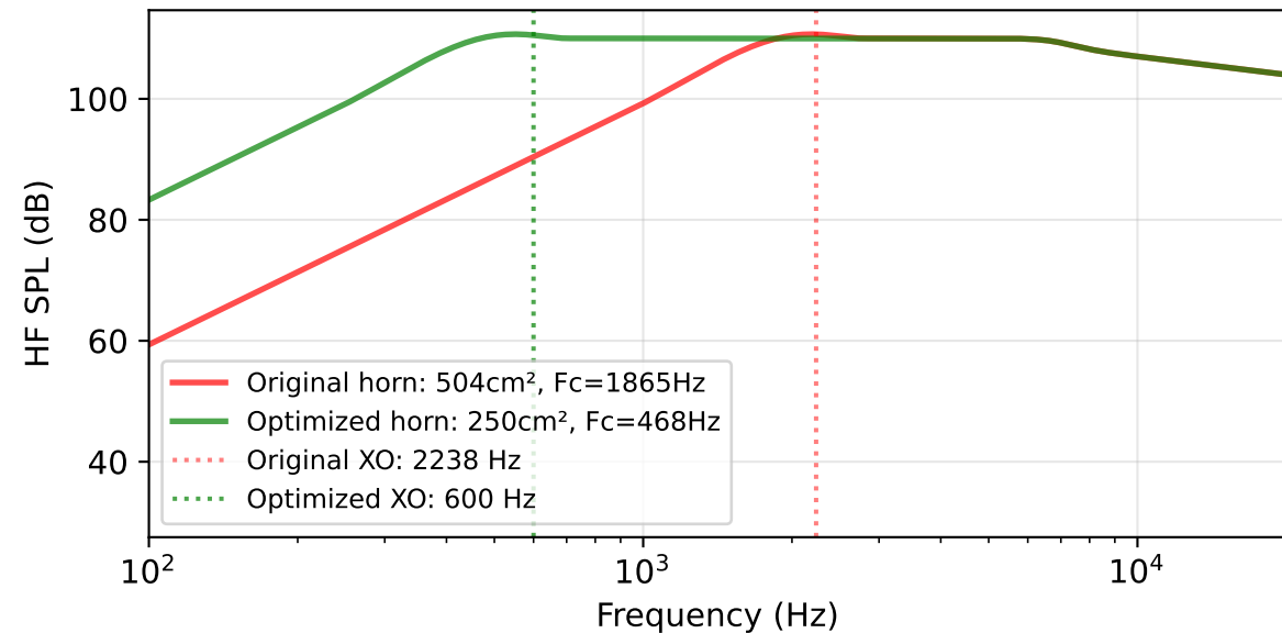
Horn Response Comparison (raw, before padding)
