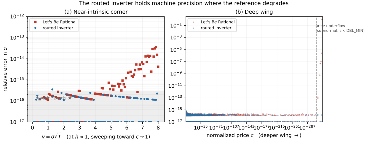
Figure 5: Relative error in \sigma in the two regimes where the reference degrades. (a) Near the intrinsic value, at h \approx 1 as c \rightarrow 1 , LBR climbs toward 10^{-13} from the conditioning of its normalized objective, while the routed inverter stays at machine precision. (b) In the deep wing, once the price is subnormal the reference’s reduced variable \beta = c e^{-h/2} underflows and it loses precision, whereas the routed inverter, working in c , does not.
