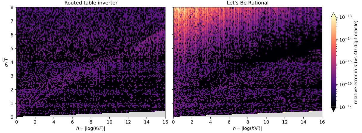
Figure 4: Relative error in \sigma against the 40-digit oracle over the (h, \sigma\sqrt{T}) domain. The routed table inverter (left) is uniformly at machine precision. LBR (right) degrades in the near-intrinsic upper-left corner and, more mildly, in the deep wing. Grey marks prices that round to 0 or 1 in double precision.
