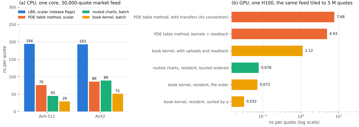
Figure 1: Cost per quote of every method on the same market feed, a tradeable 2024 S&P 500 book of 30,000 quotes. (a) One CPU core, all methods in one binary timed by the same loop on a quiet host (Table 4): the reference LBR at its author’s release flags, the PDE table method, and the batch paths of the routed charts and of the book kernel. (b) One NVIDIA H100 on the feed tiled to about five million quotes (Table 6), kernel-resident and, where marked, with the host transfers of the PDE method’s own timing convention. LBR, the routed charts and the book kernel all hold machine precision on this feed (worst relative error in \sigma below 10^{-15} against a 40-digit oracle), and every result of ours is bit-identical to the scalar entry on every quote. The PDE table method does not: its worst error on the same feed is 1.2 \times 10^{-5} , ten orders of magnitude larger.
