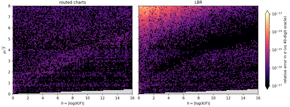
Figure 6: Relative error in \sigma against the 40-digit oracle over the regular grid, the routed charts alone (left) and LBR (right), both called from the same (h, c) pairs as Table 6. The routed charts are uniformly at machine precision. LBR degrades toward the near-intrinsic corner ( v \rightarrow 8 , small h ) and along the lower edge of the wing, where its reduced variable underflows. Grey marks prices that round to 0 or 1 in double precision.
