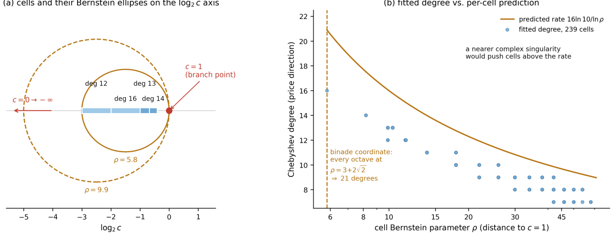
Figure 5: The branch-point geometry that sizes the tabulated chart. (a) The cells nearest the money in one h -band of the table on the \log_2 c axis, with the Bernstein ellipses of two cells drawn in place. Each cell’s largest singularity-free ellipse passes through the c = 1 branch point, so \rho grows as cells recede from the money, and sub-splitting the octaves adjacent to the money (dark cells) keeps \rho \geq 3 + 2\sqrt{2} for every cell. (b) The fitted price-direction degrees of all 239 cells against \rho , with the predicted rate 16 \ln 10 / \ln \rho overlaid. The degrees track the rate from below at a uniform offset (Appendix D.1), and no cell sits systematically above it, as a nearer complex singularity would force.
