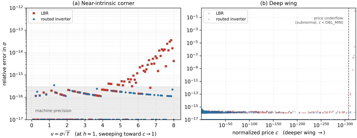
Figure 7: Relative error in \sigma in the two regimes where the reference degrades. (a) Near the intrinsic value, at h \approx 1 as c \rightarrow 1 , LBR climbs to 3.6 \times 10^{-14} from the conditioning of its normalized objective, while the routed inverter stays below 4 \times 10^{-16} . (b) In the deep wing both hold machine precision across three hundred orders of magnitude of the price, until the reference’s reduced variable \beta = c e^{-h/2} becomes subnormal and it loses precision, whereas the routed inverter, working in c , holds to the last representable price.
