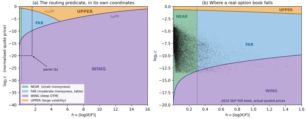
Figure 4: Routing of the input domain in the coordinates the classifier uses. (a) The strip 0 < c < 1 of normalized quote prices against moneyness h = |\log(K/F)| , tiled by the four charts. Each seam is a threshold price returned by a frozen polynomial in h , c_w(h) = C(h, h/\sqrt{7.6}) below and c_{top}(h) = C(h, 1.85) above, so the two curves are the routing predicate itself, and every point of the strip is a genuine quote. (b) The near-the-money corner (boxed in (a)) with a year of tradeable 2024 S&P 500 quotes overlaid at their actual quoted prices. About 92% of the book falls in the small-moneyness chart and 7% in the tabulated chart, and the large-volatility region carries none.
