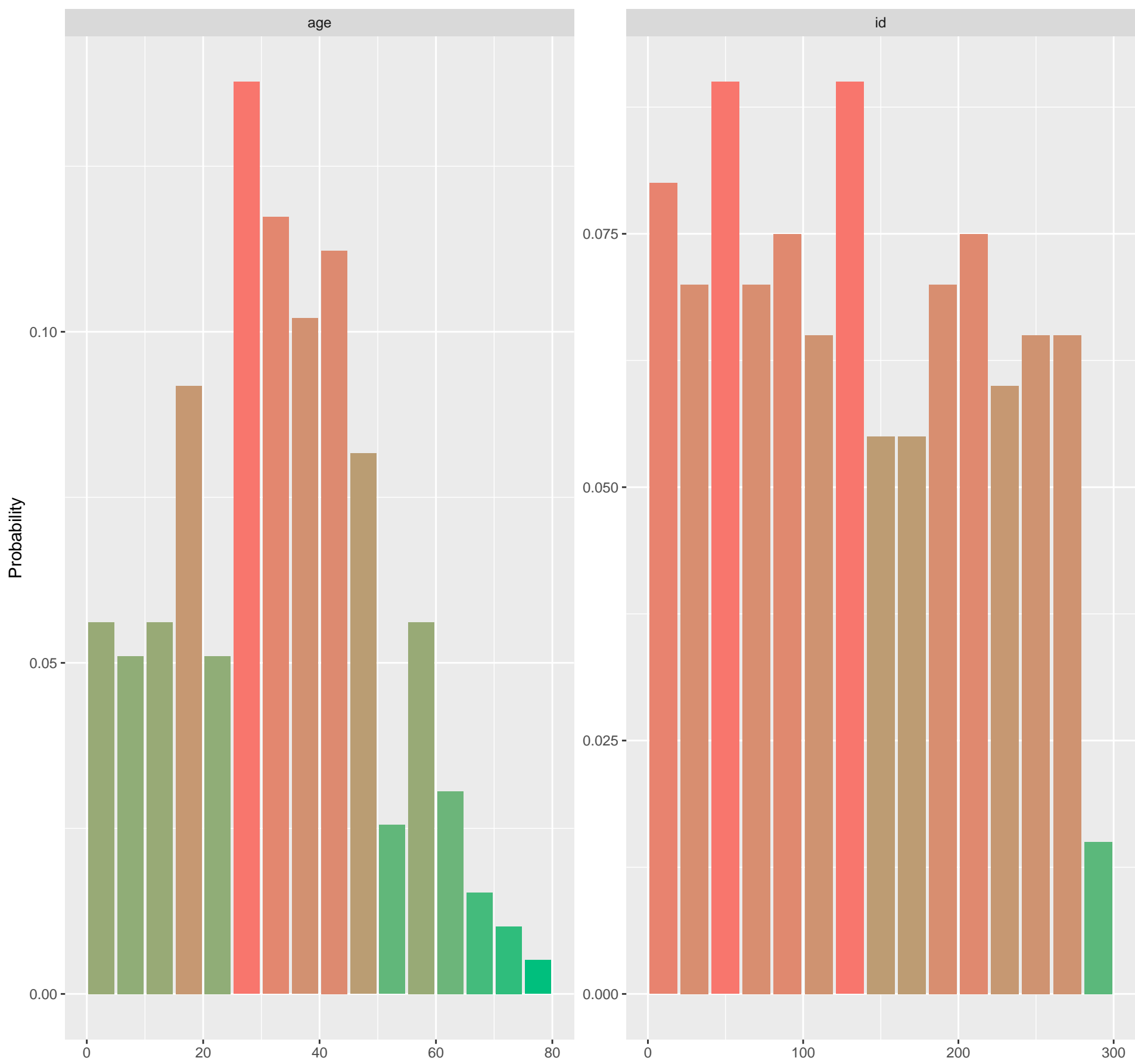
Histograms of numeric columns in df::ebola_data
