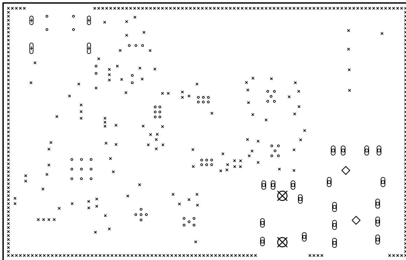
Drill Map:
