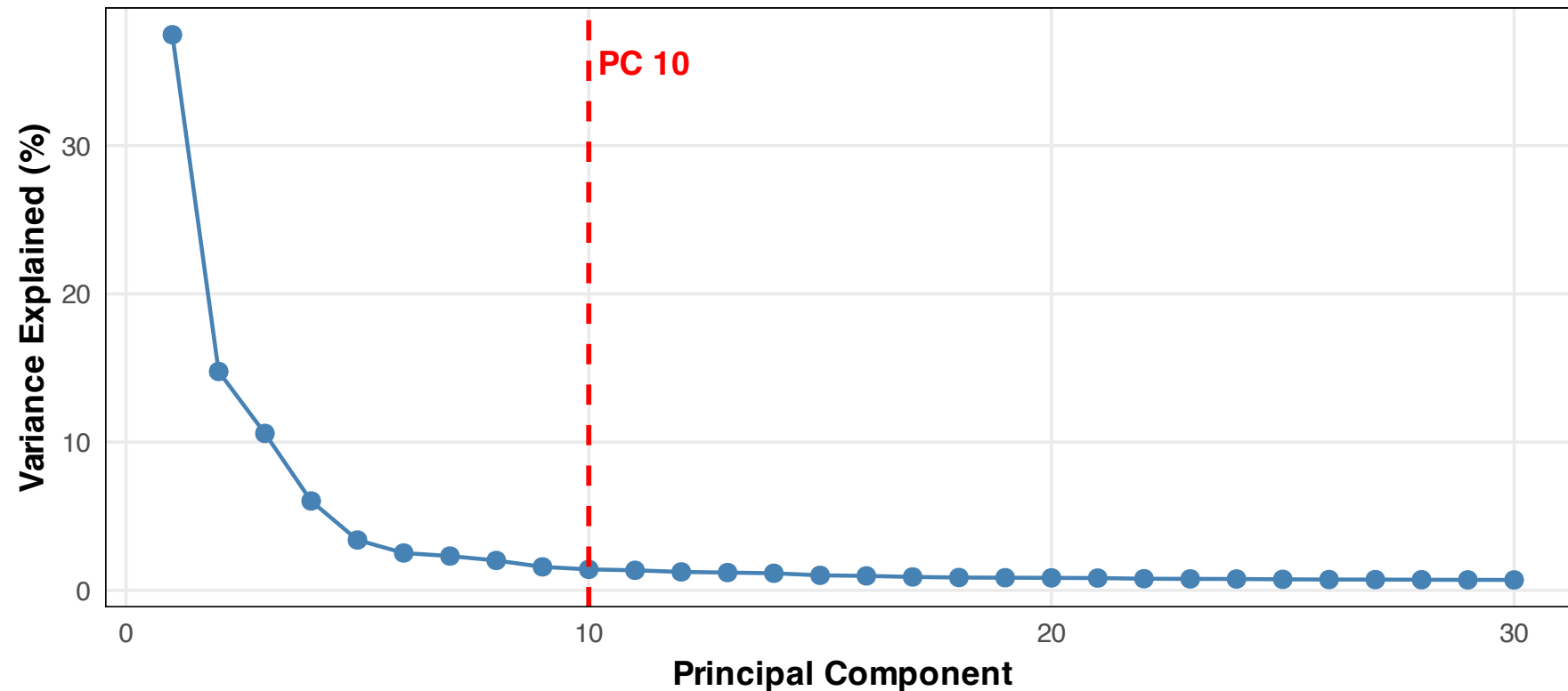
PCA Variance Explained by Each Principal Component
