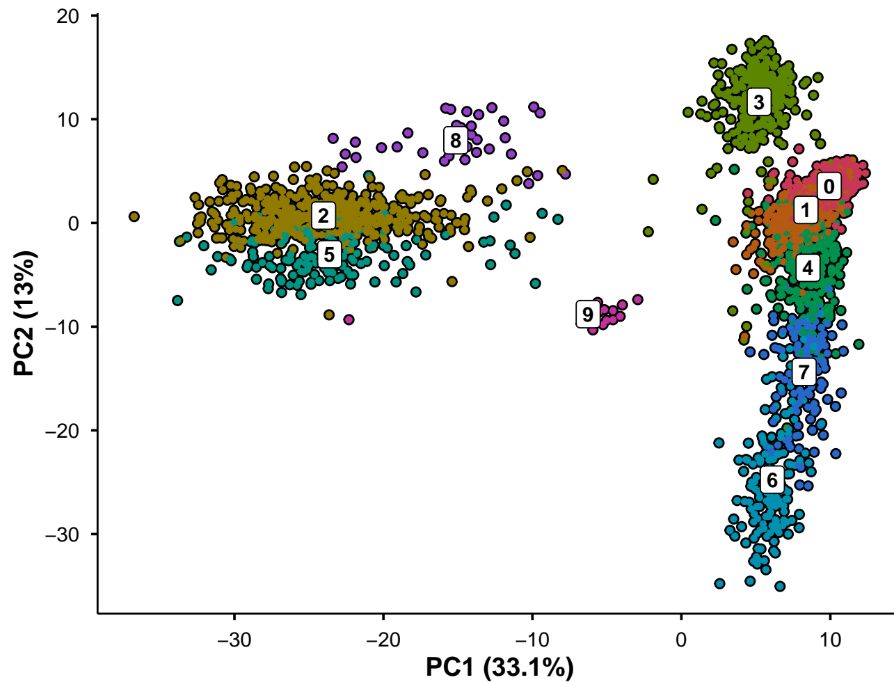
PC1 vs PC2
