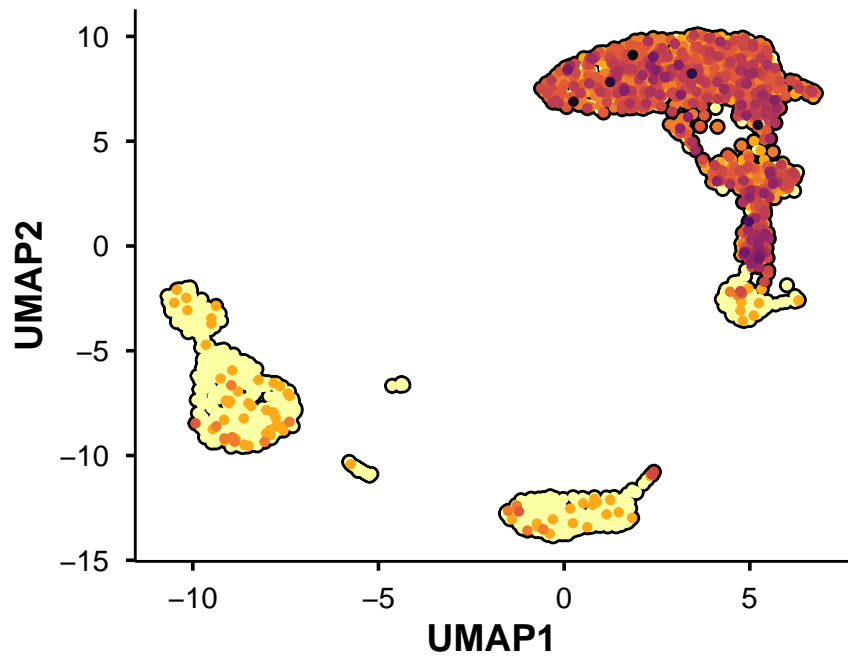
CD3D
