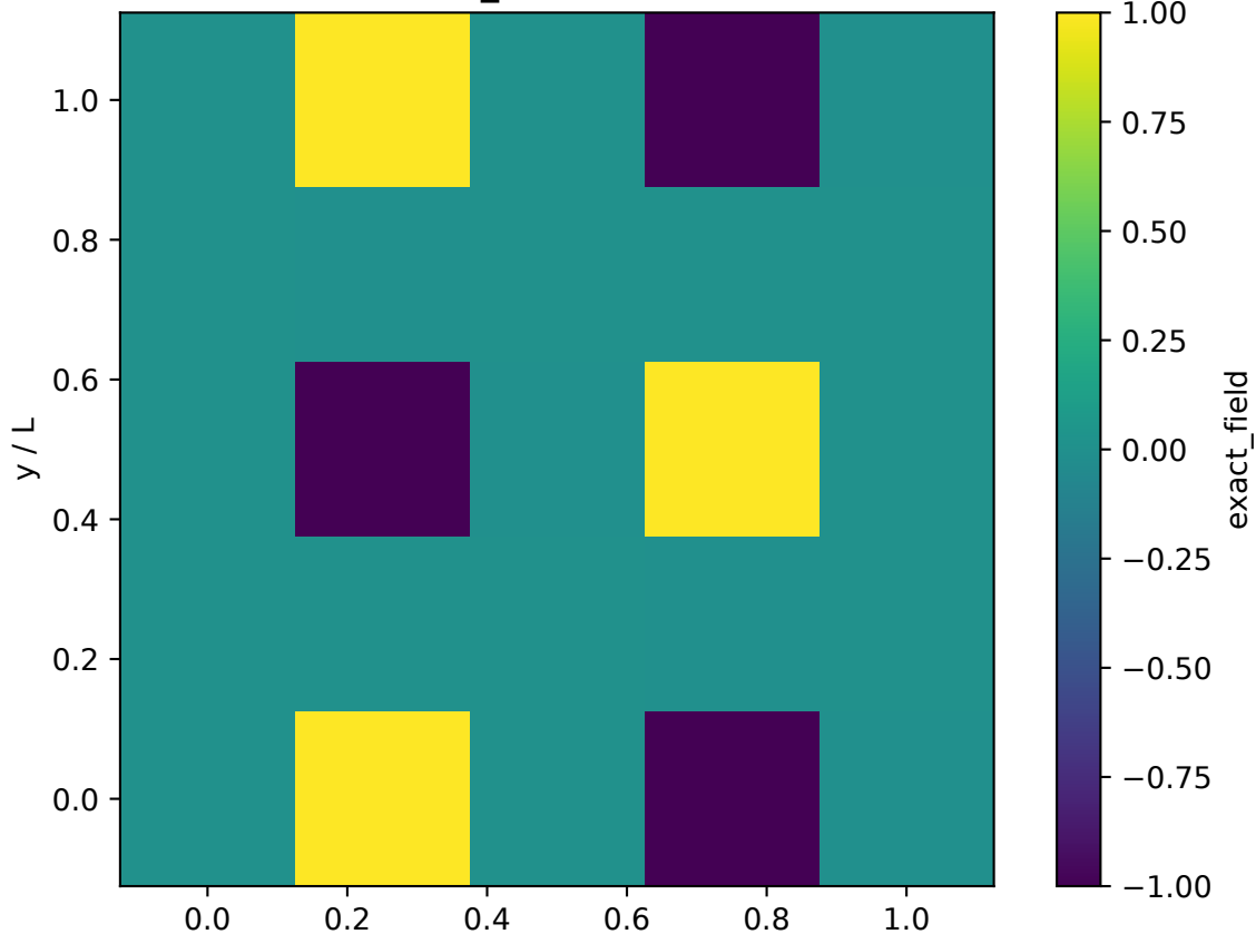
exact_field (fixture)
