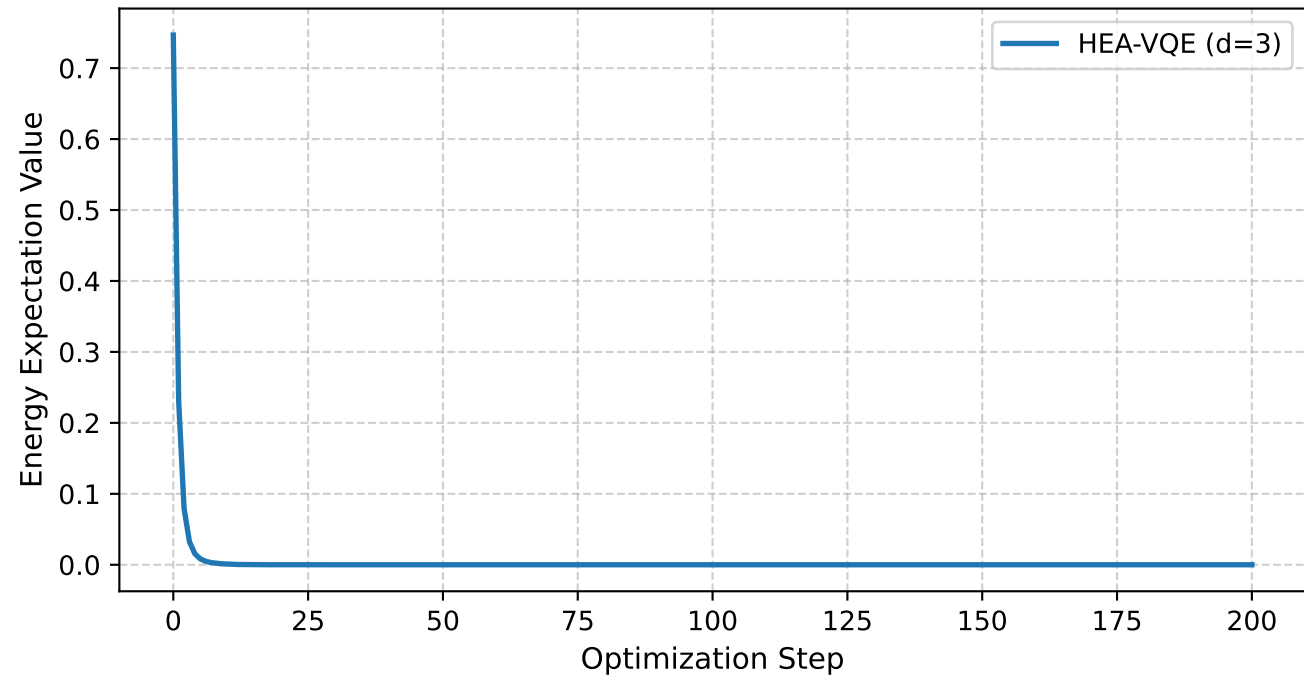
Energy Convergence on 12-Qubit 3-Regular Max-Cut
