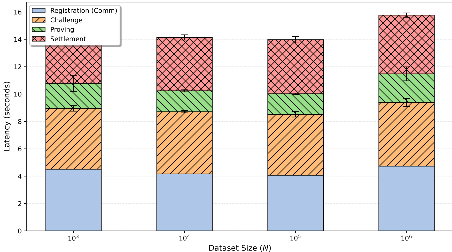
End-to-End Latency Breakdown of Block-Sampling Protocol
