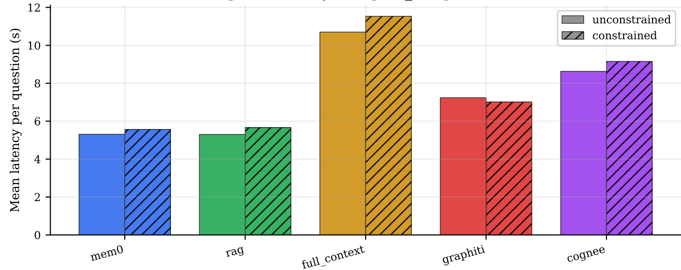
Ask-phase latency (compute_ms) per backend
