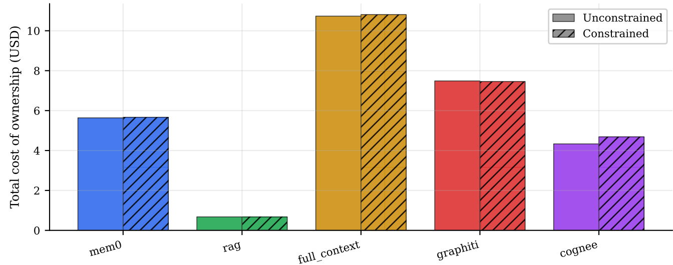
Total TCO per backend — load + ask (AWS Fargate us-east-1)
