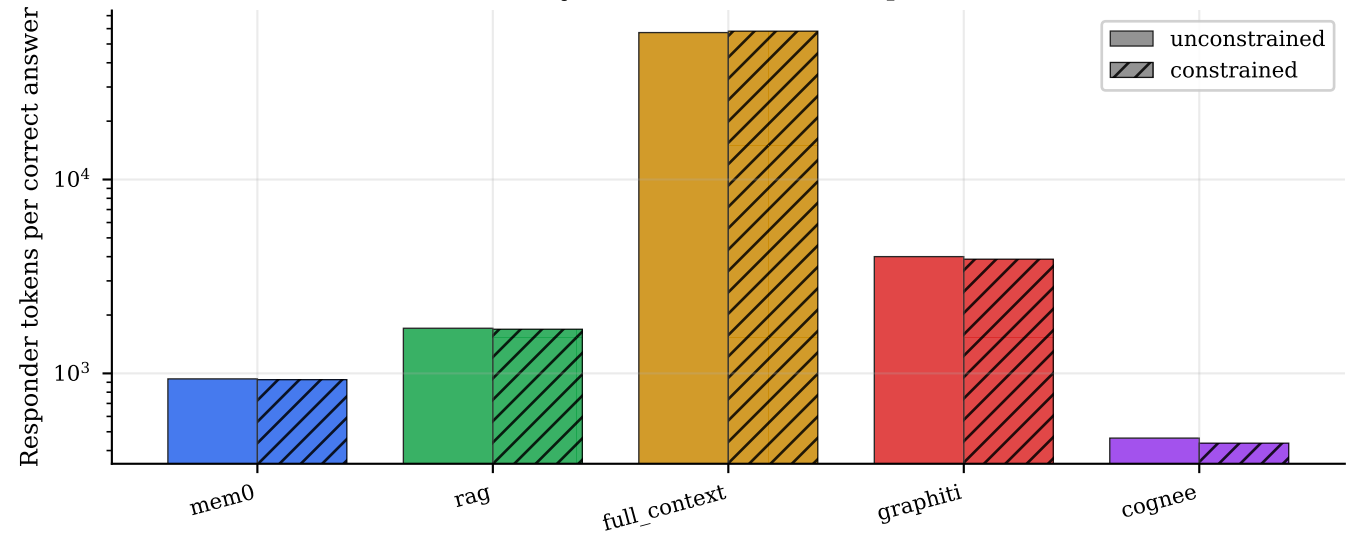
Retrieval efficiency — tokens consumed per correct answer
