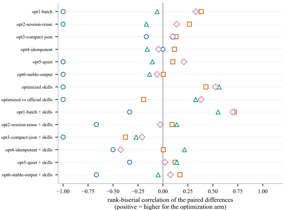
Optimization arm vs like for like CLI baseline
