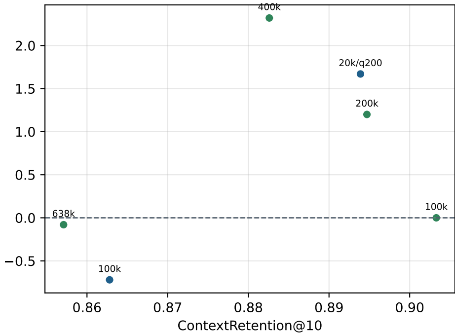
IntentRoute Hit@10 delta vs dense (pp)
