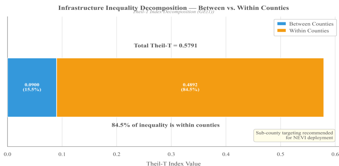
Figure 33 Theil-T Decomposition of EV Charging Infrastructure Inequality: Within-County vs Between-County
