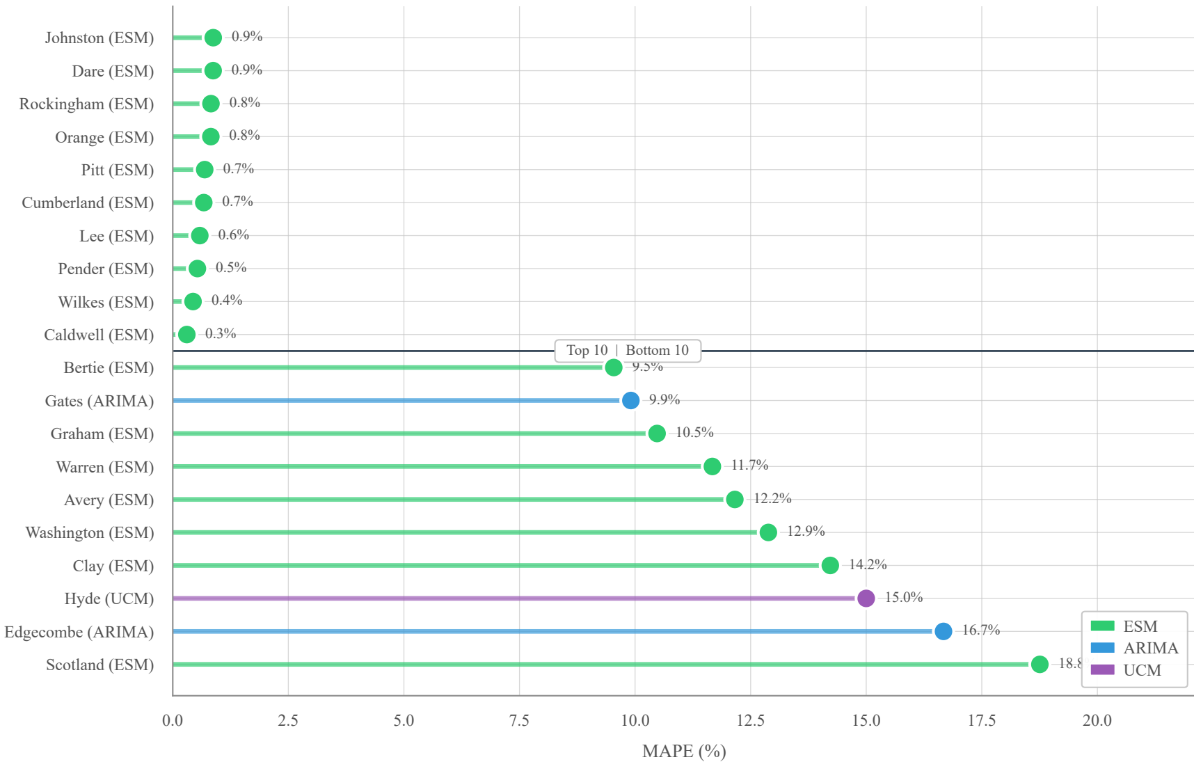
County Forecast Performance: Top 10 vs Bottom 10
