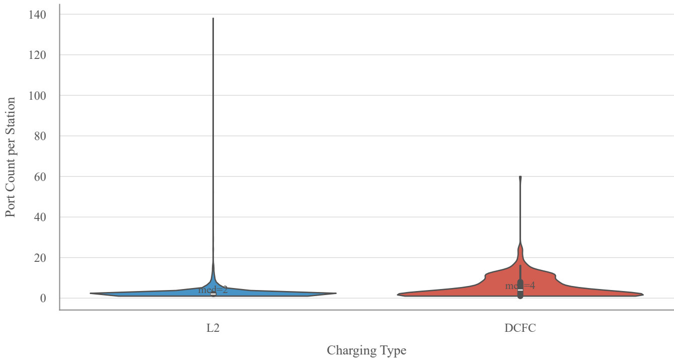
Port Count Distributions (L2 vs DCFC)
