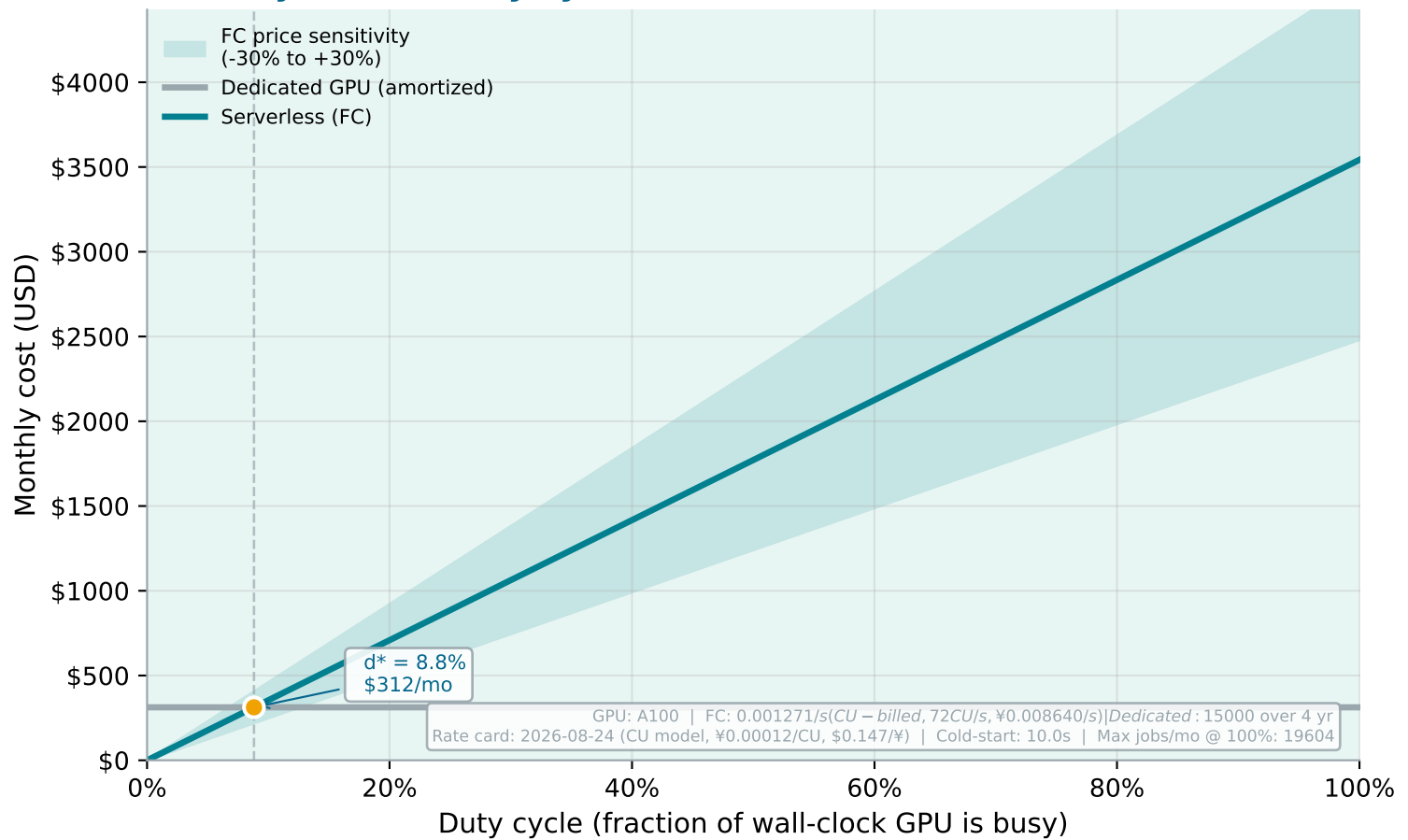
Monthly cost vs duty cycle
