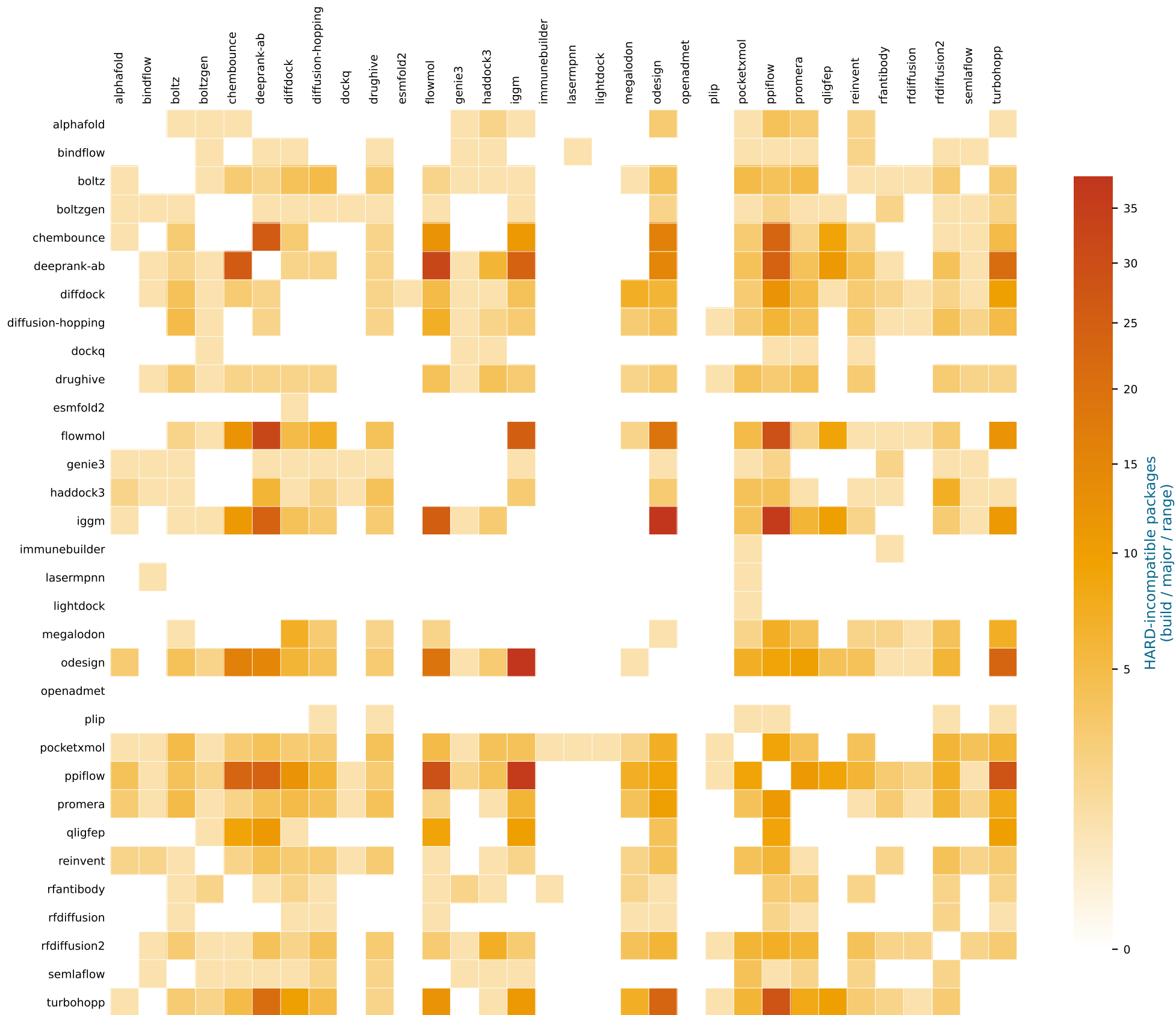
Conflicts — HARD-incompatible packages per service pair
