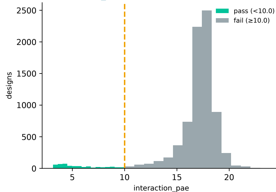
interaction_pae < 10.0 (490/8000 pass)
