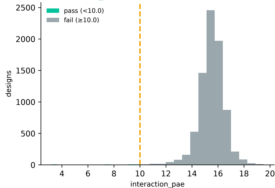
interaction_pae < 10.0 (47/8000 pass)
