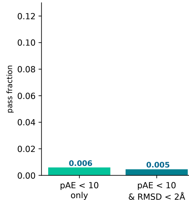
filter contribution
