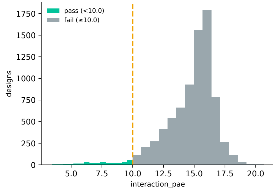
interaction_pae < 10.0 (317/8000 pass)
