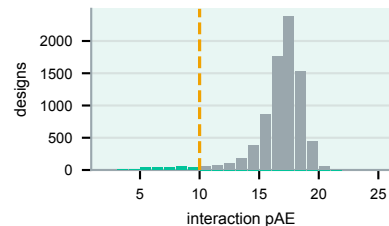
TcdB scFv unique (200/8000 < 10)
