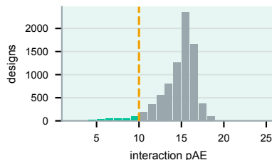
TcdB scFv comb. (866/8000 < 10)
