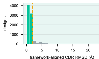
TcdB scFv unique (3319/8000 < 2)
