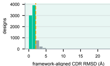
TcdB (6923/8000 < 2)
