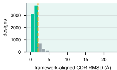
RSV-F Site I (6555/8000 < 2)
