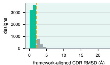
SARS-CoV-2 RBD (7246/8000 < 2)
