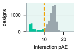
pAE (1693/8000 < 10)
