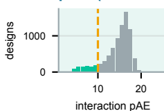
pAE (866/8000 < 10)
