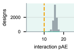
pAE (47/8000 < 10)
