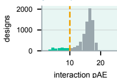
pAE (845/8000 < 10)
