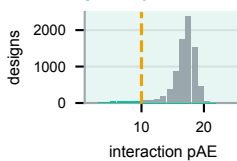
pAE (200/8000 < 10)
