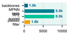
TcdB funnel
