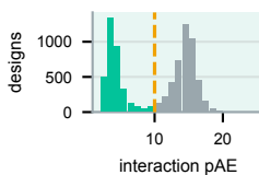
pAE (3484/8000 < 10)
