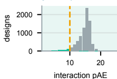
pAE (317/8000 < 10)
