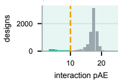
pAE (490/8000 < 10)
