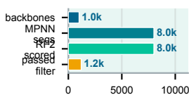
IL-7Ra funnel
