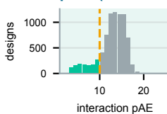
pAE (1235/8000 < 10)
