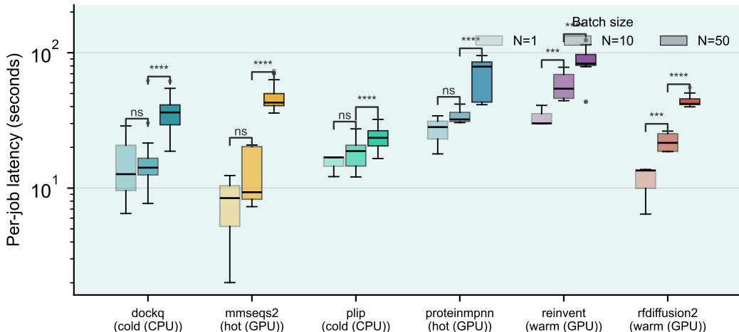
(a) Per-Job Latency Distribution — grouped by service
