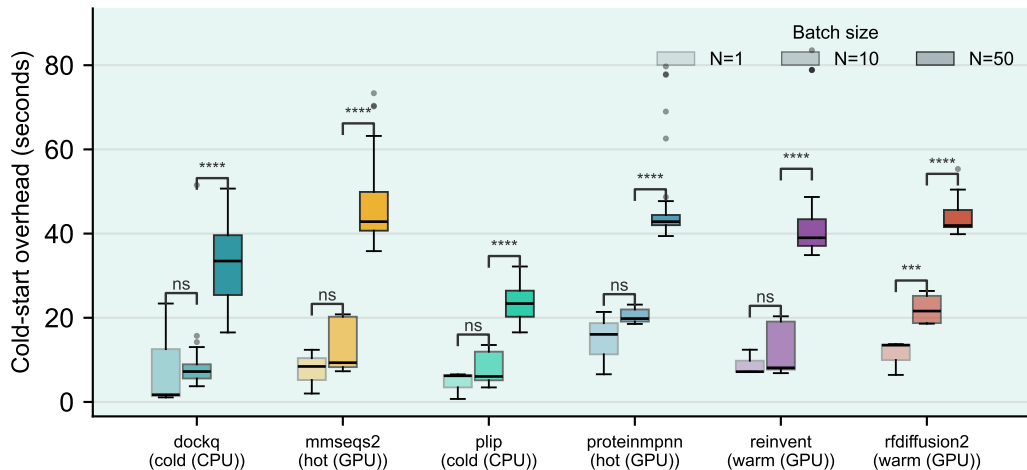
(b) Cold-Start Overhead (submit → running) — grouped by service
