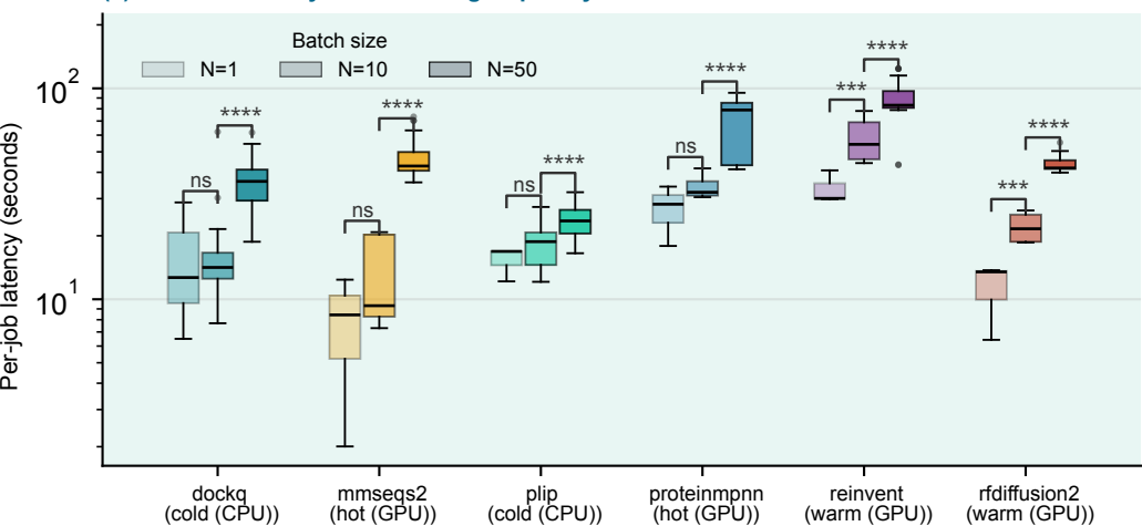
(a) Per-Job Latency Distribution grouped by service
