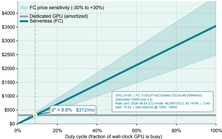
Monthly cost vs duty cycle
